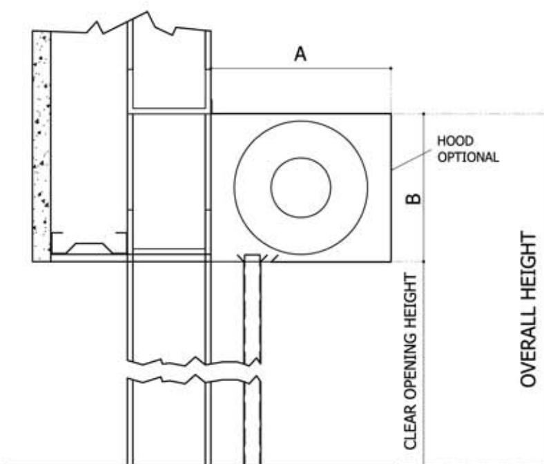
SECTIONAL ELEVATION
